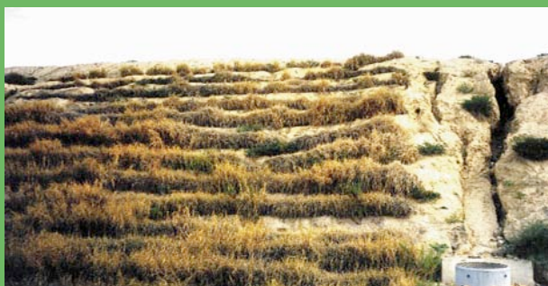
Spain - unstable and eroding highway fill treated with VS. Untreated eroded fill on right. VS grows well under low rainfall Mediterranean climate
